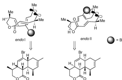
Scheme 2. Comparison of endo transition states.
